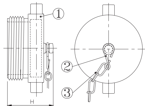
DIMENSIONS Unit: inch
